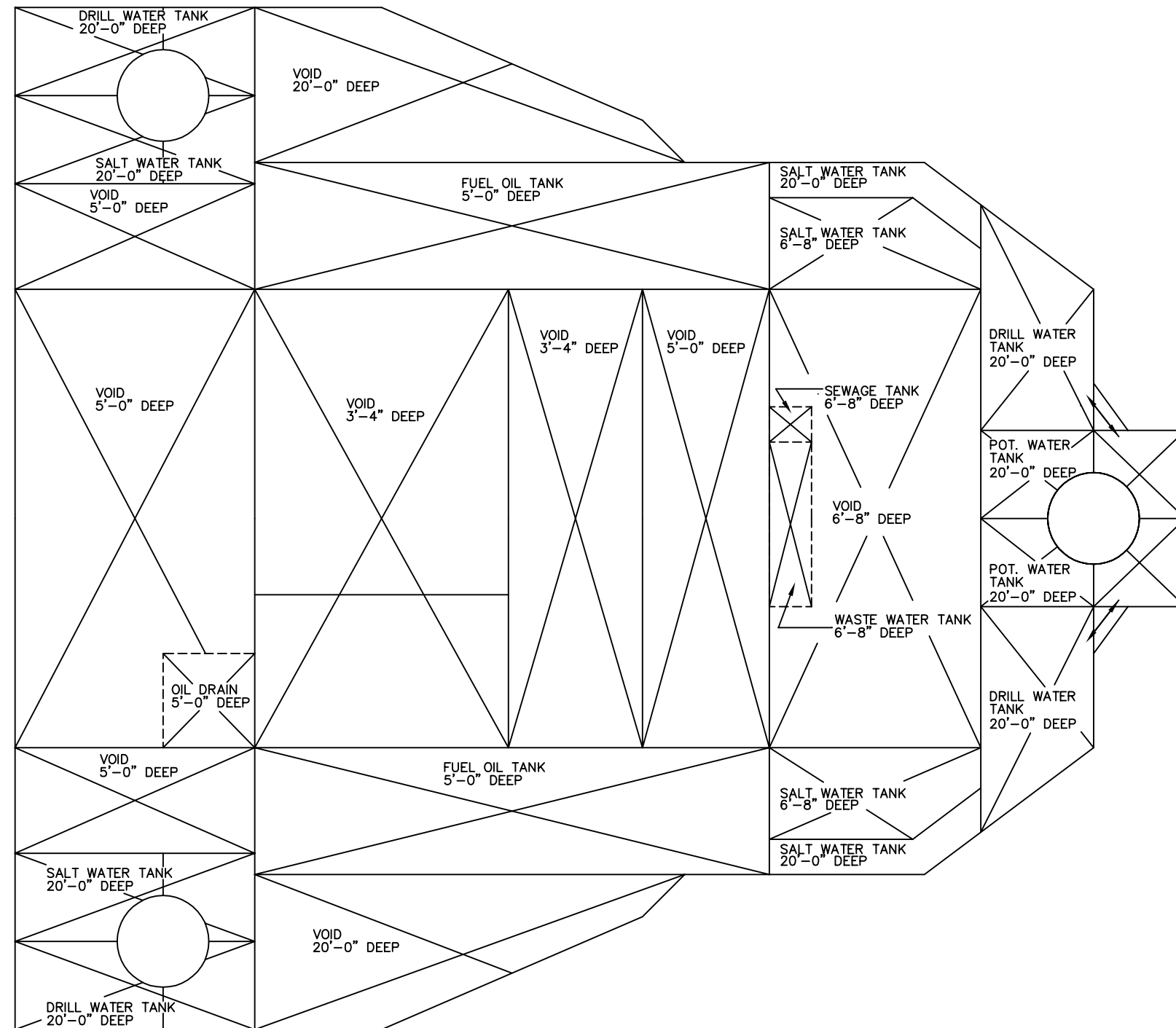
PLATFORM TANKS SCALE: 3/64" = 1'-0"
