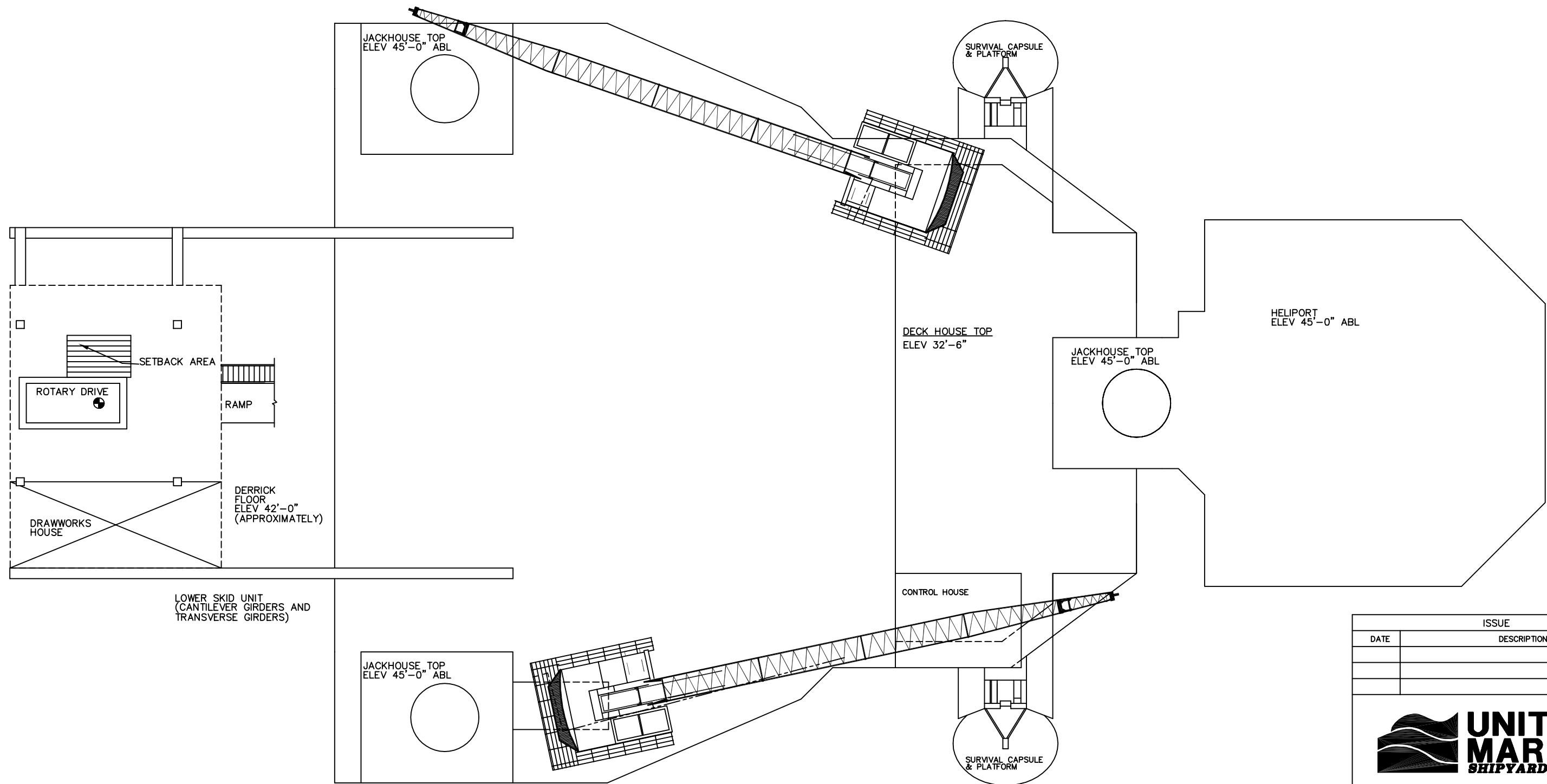
PLAN OF HELIPORT, HOUSETOP & SKID UNIT
