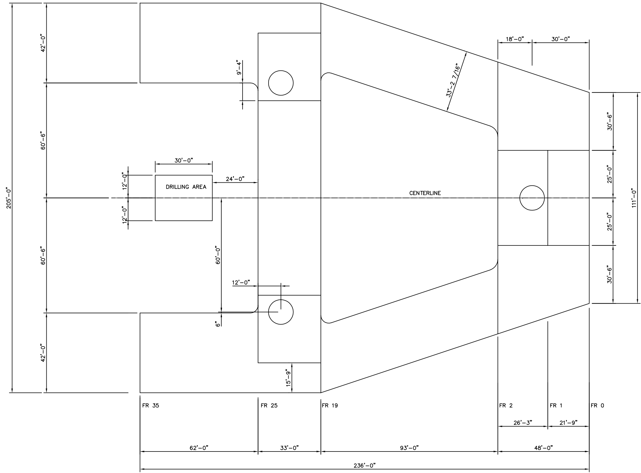
MAT DIMENSION PLAN SCALE: 1/32" = 1'-0"
