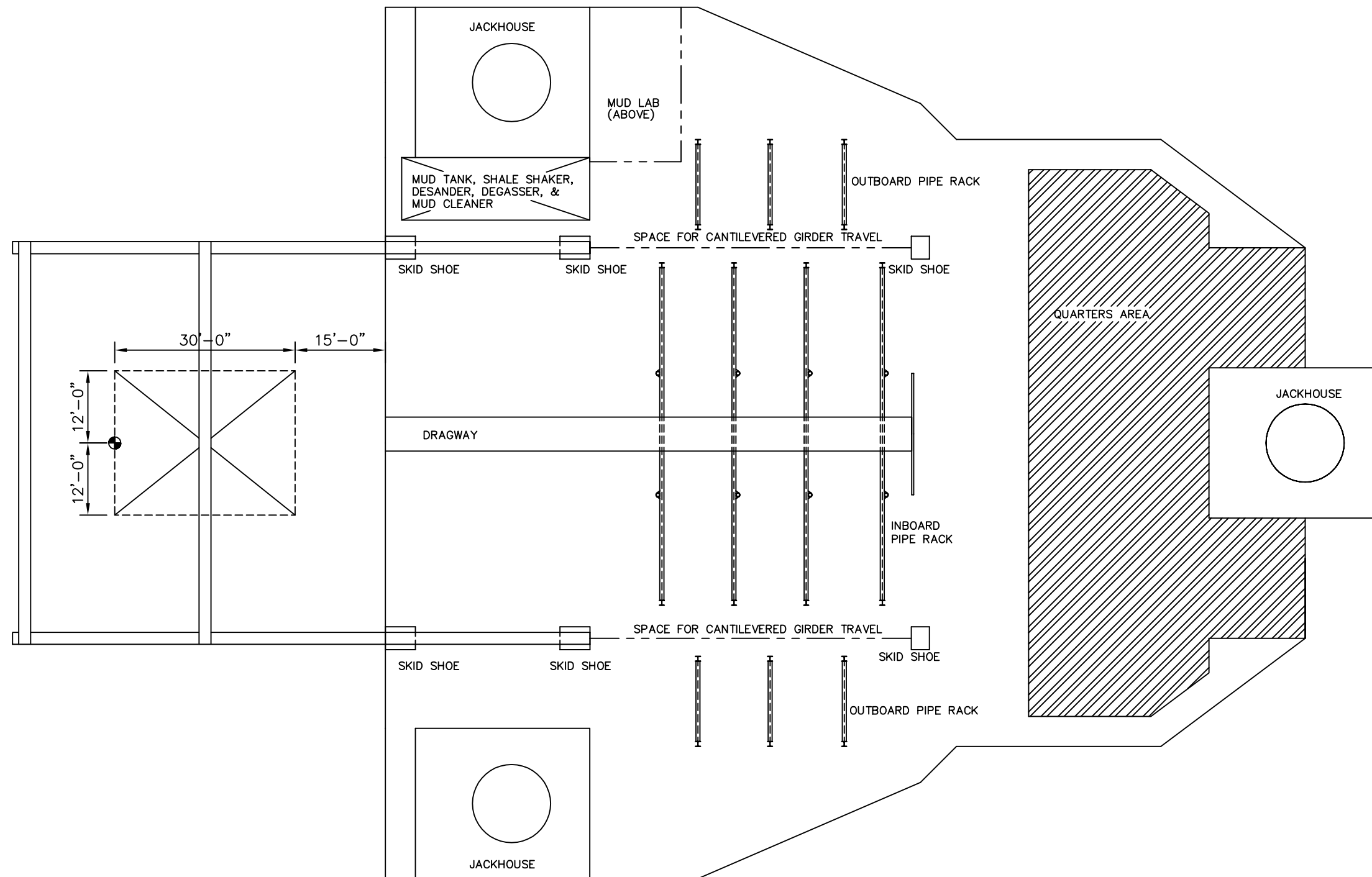
PLAN OF MAIN DECK
