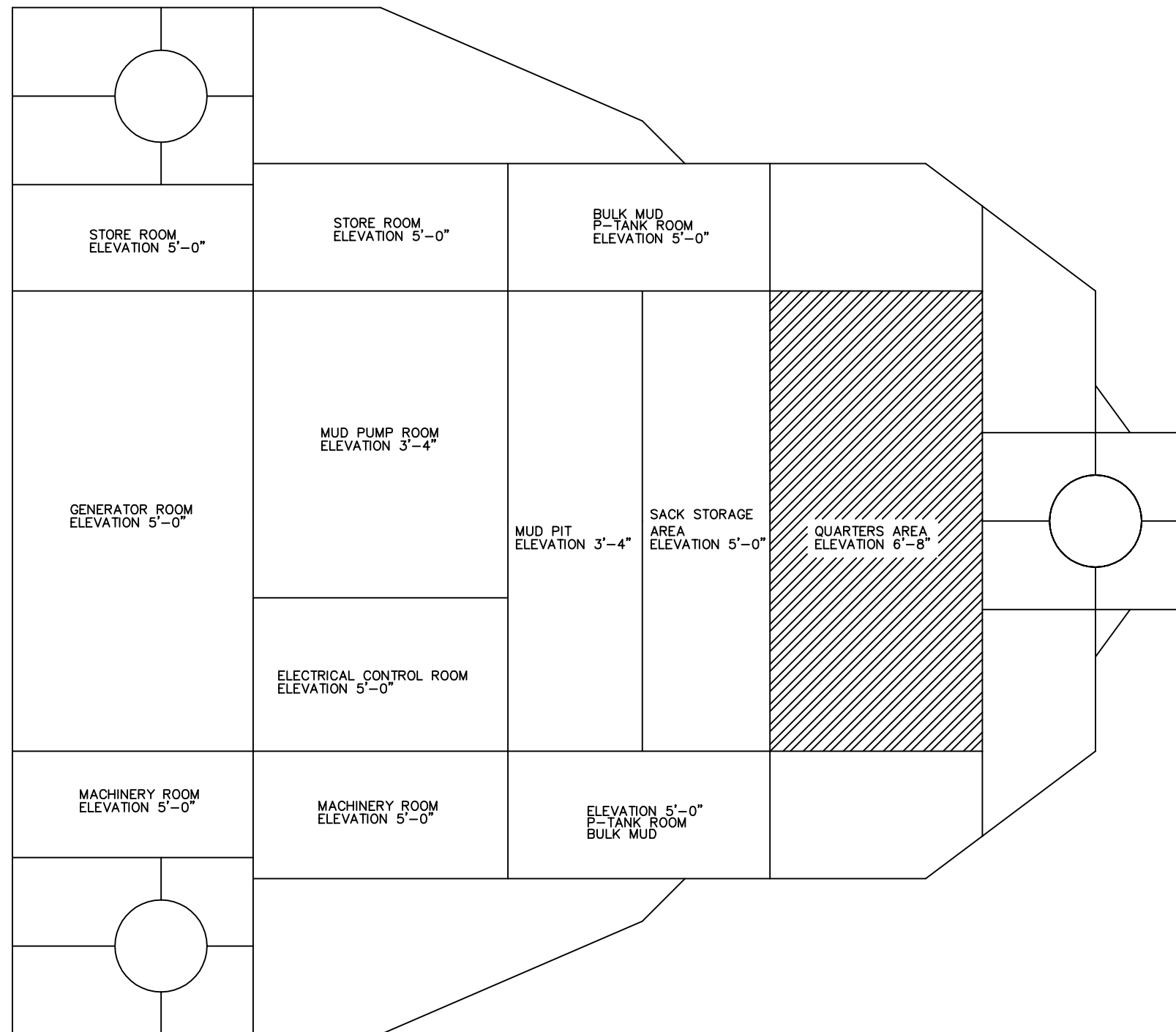
PLAN OF PLATFORM LOWER DECK
