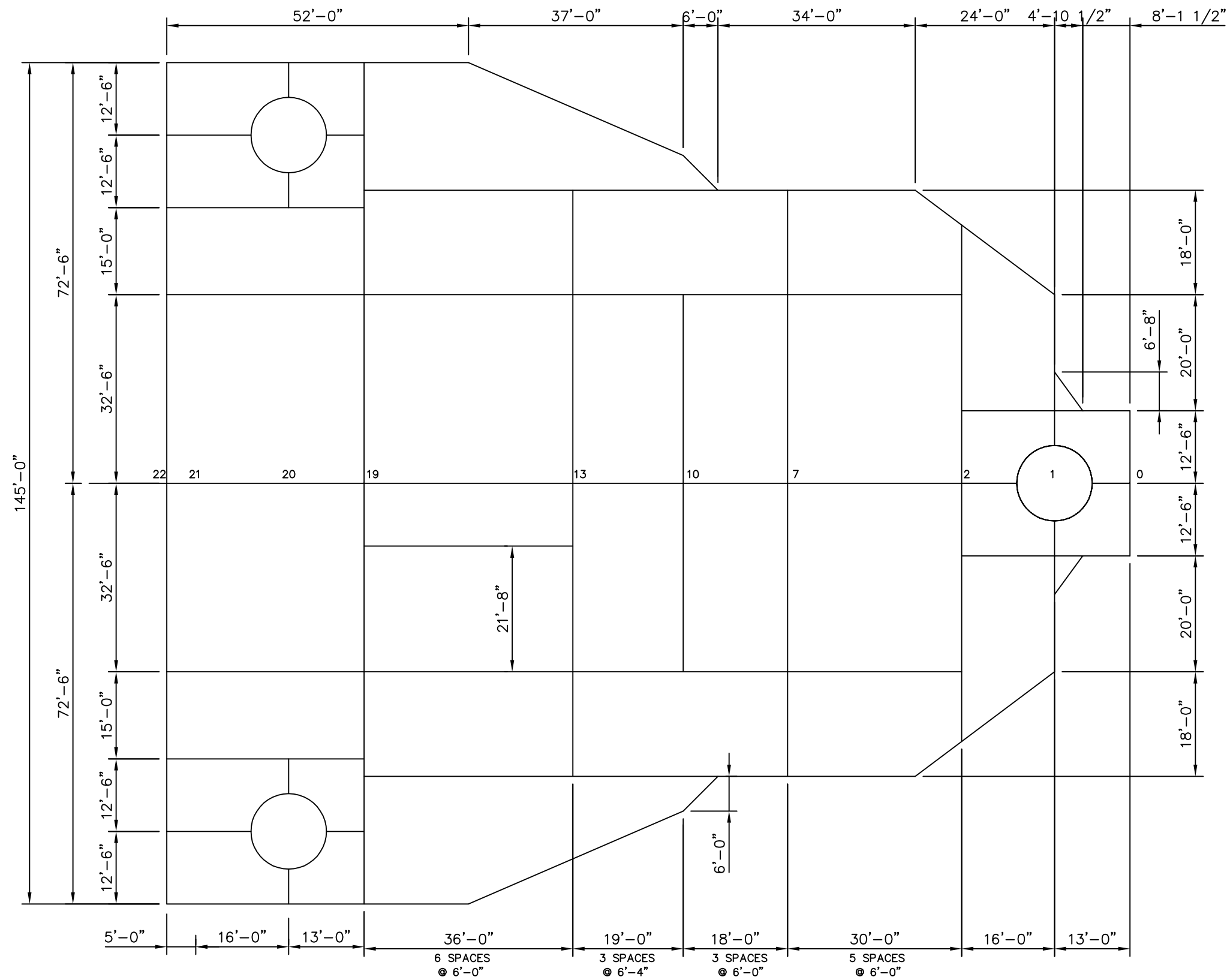
PLATFORM DIMENSION PLAN SCALE: 3/64" = 1'-0"
